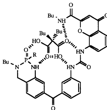
Figure 4. Complex for Receptor 11 and DBMA.
