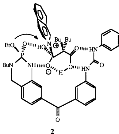
Figure 3. Proposed Transition State Complex for Decarboxylation of DBMA and Receptor 2.
