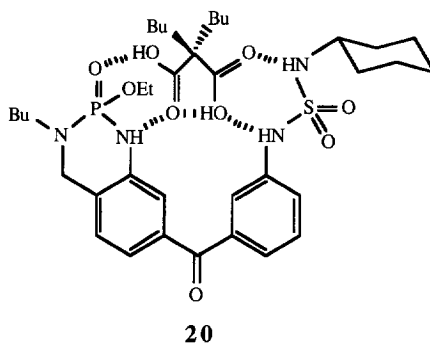
Figure 5. Receptor 20 and DBMA complex.
