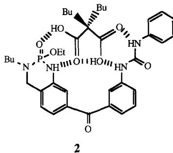
Figure 2. Proposed Complex for Receptor 2 and DBMA.
