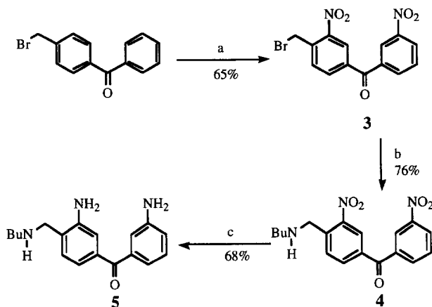
Scheme 2. Synthesis of the triamine 5 .
