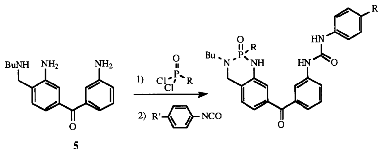
Scheme 3. General Synthesis of Receptors.
