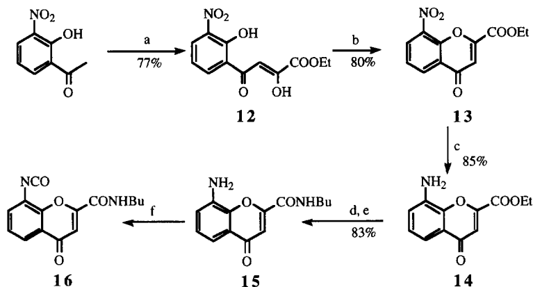
Scheme 4. Synthesis of isocyanate 16 .
