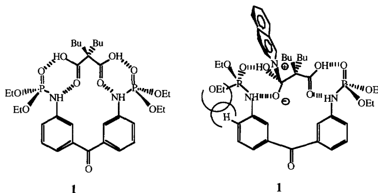
Figure 1. Proposed Complexes for Receptor 1 with Dibutylmalonic Acid (DBMA) in Ground and Transition State.
