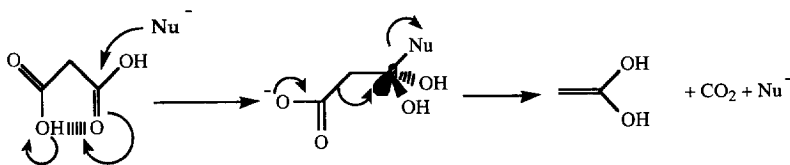
Scheme 1. Proposed Mechanism for Malonic Acid Decarboxylation.
